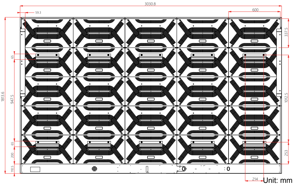
< Rear View >
