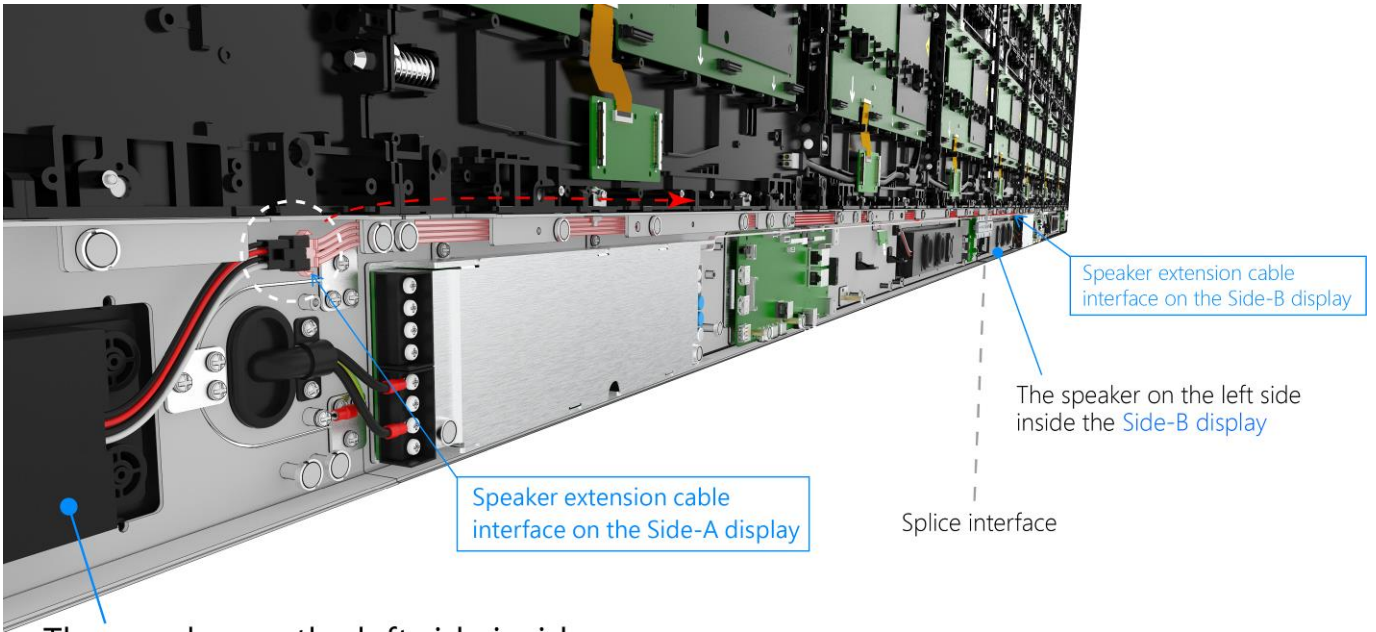
The speaker on the left side inside the Side-A display
